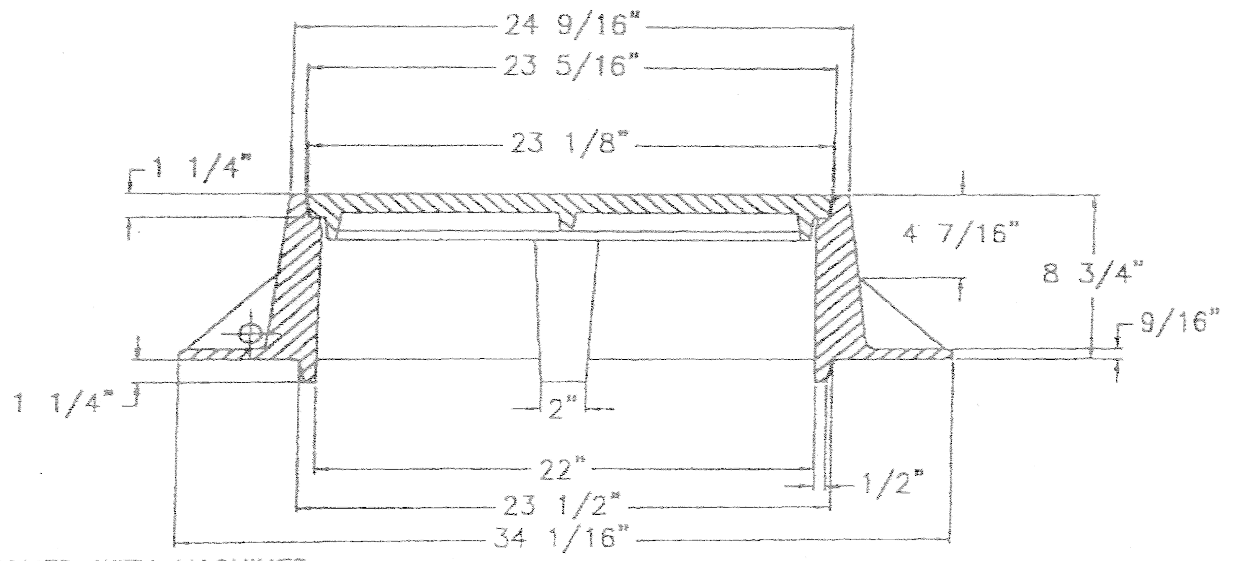
ATTACHMENT B MANHOLE RING & COVER
